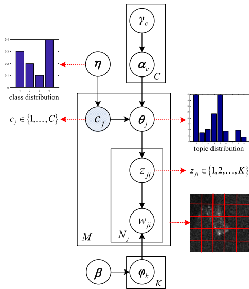
Fig. 6. Graphical model of SSILDA.
