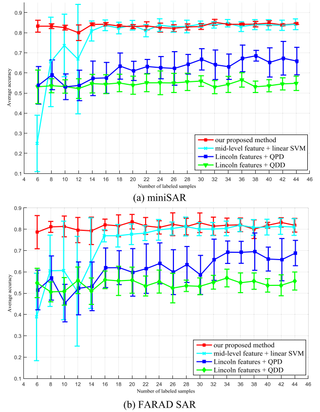
Fig. 15. Variations of average accuracy and corresponding standard deviation via different supervised methods with the number of labeled samples. (a) Results on the miniSAR data set. (b) Results on the FARAD SAR data set.
