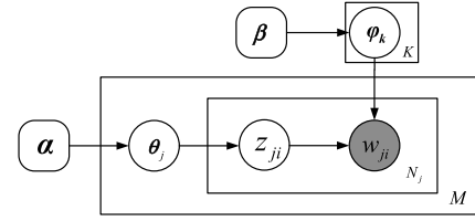
Fig. 1. Original LDA proposed in [21].
