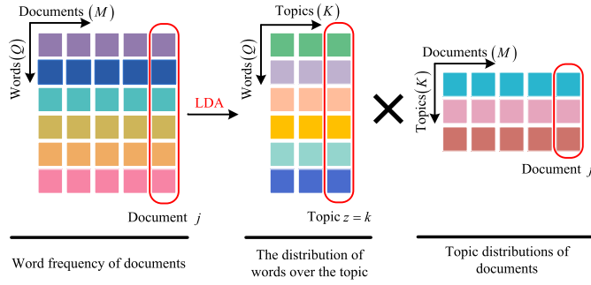
Fig. 2. Topic representation process of the LDA model.
