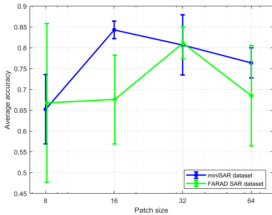
Fig. 9. Variation of average accuracy and standard deviation with the patch size.
