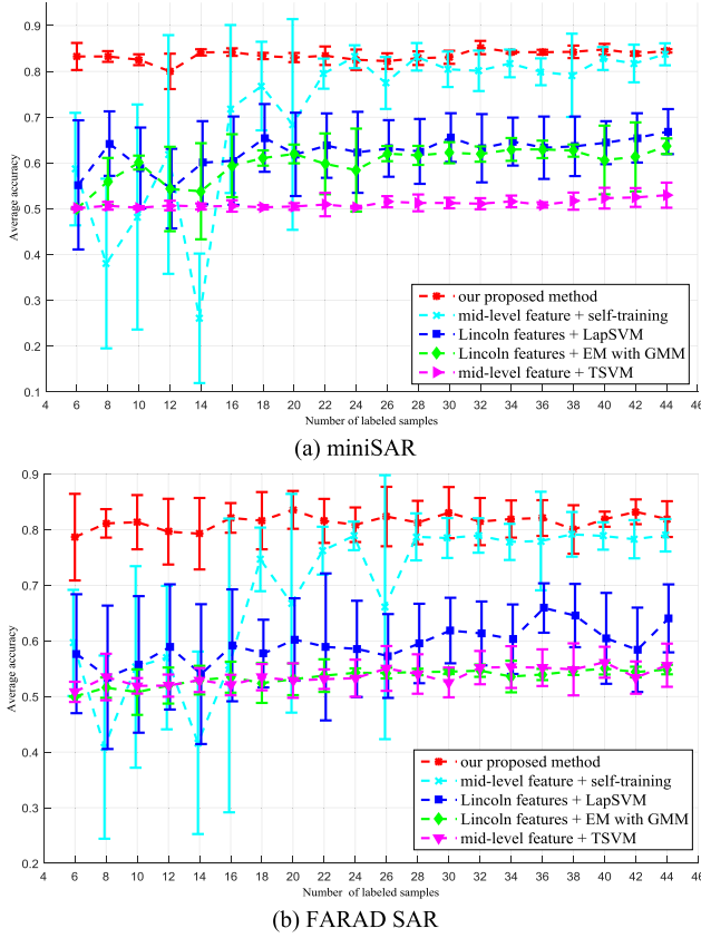
Fig. 14. Variations of average accuracy and corresponding standard deviation via different semisupervised methods with the number of labeled samples. (a) Results on the miniSAR data set. (b) Results on the FARAD SAR data set.
