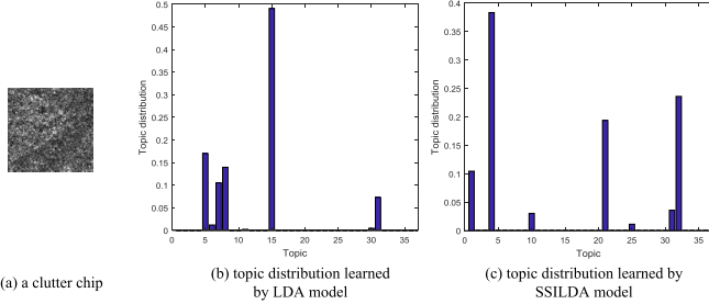
Fig. 12. (a) Clutter chip and its topic distributions learned by the (b) LDA model and (c) SSILDA model.
