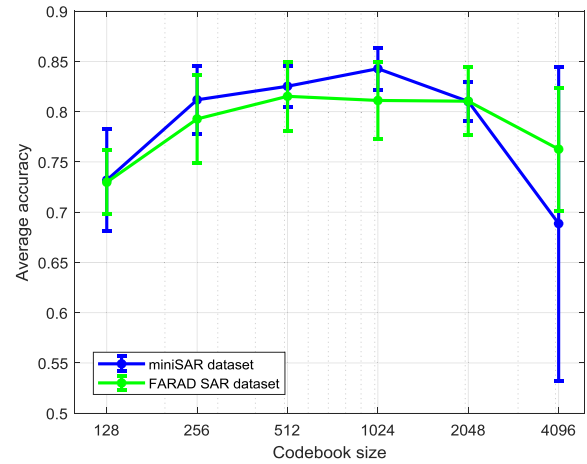
Fig. 10. Variation of average accuracy and standard deviation with the codebook size.
