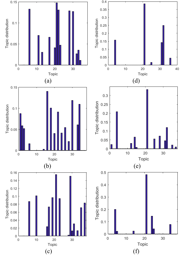
Fig. 13. Topic distribution examples of target and clutter chips. (a)–(c) Topic distributions of three target chips. (d)–(f) Topic distributions of three clutter chips.
