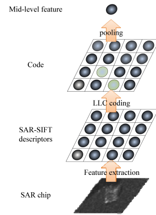
Fig. 4. Generation process of mid-level feature based on the BoVW model.
