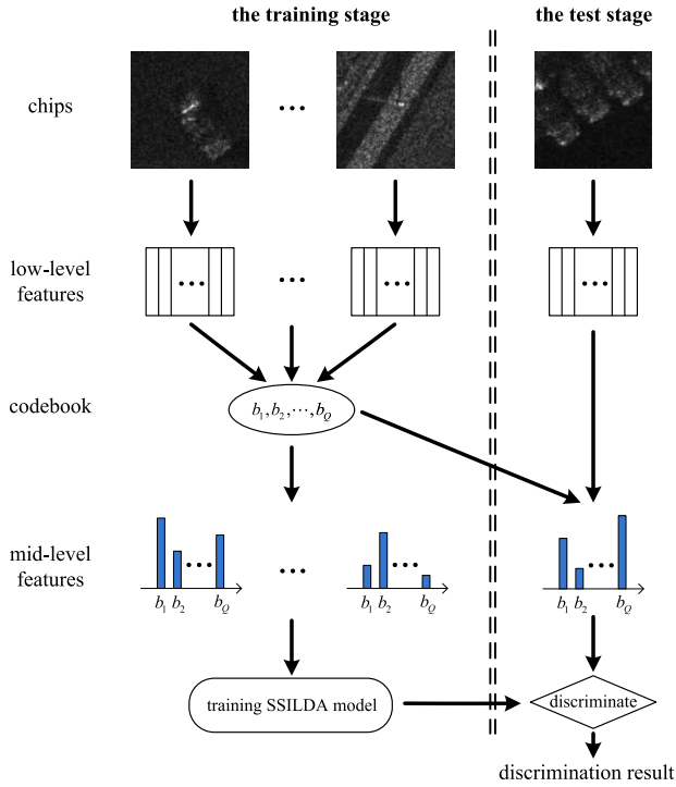
Fig. 5. Framework of our proposed semisupervised target discrimination method.
